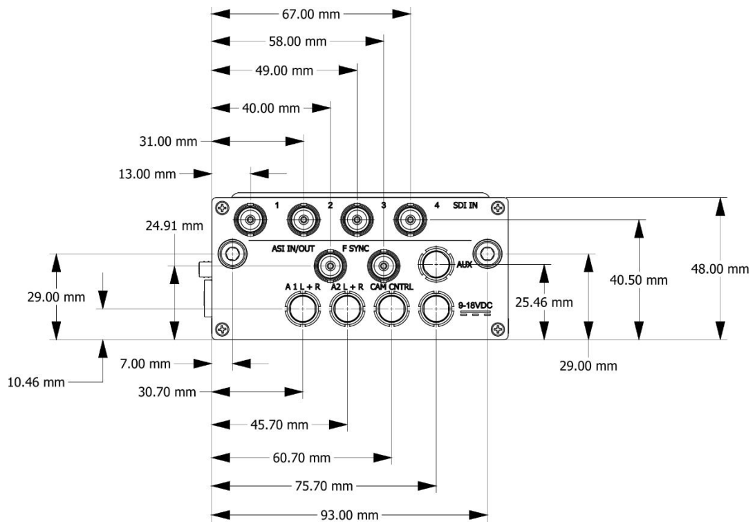
Figure 6: 4K camera back transmitter I/O module connections
