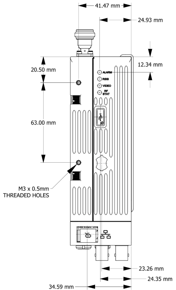
Figure 9: 4K camera back transmitter (left side)
