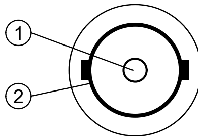
Figure 12: Front face of the BNC (F) video input connector
