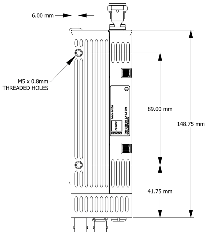
Figure 8: 4K camera back transmitter (right side)
