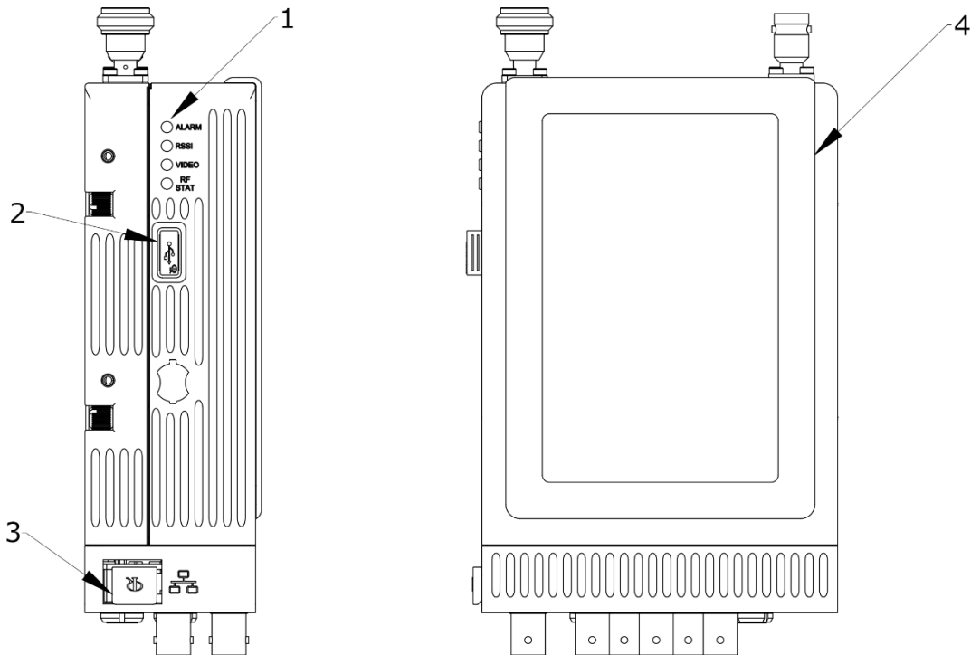
Figure 2: Connectors and components on the front and side of the 4K camera back transmitter
