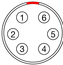
Figure 14: Front face of the LEMO audio connector
