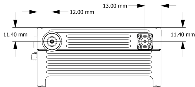
Figure 5: 4K camera back transmitter (top)
