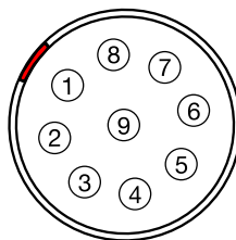
Figure 15: Front face of the LEMO AUX connector
