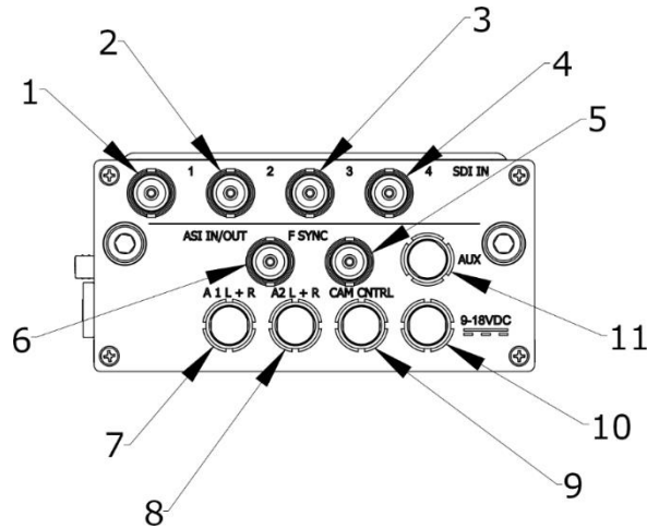
Figure 3: Connectors on the 4K camera back transmitter's I/O module
