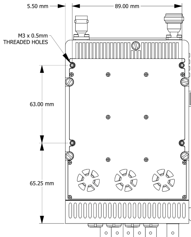
Figure 4: 4K camera back transmitter (back)
