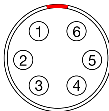
Figure 13: Front face of the LEMO audio connector
