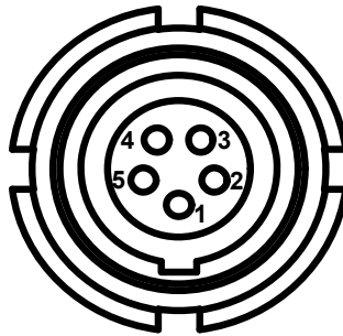
Figure 16: Front face of the LEMO 5-pin camera control connector
